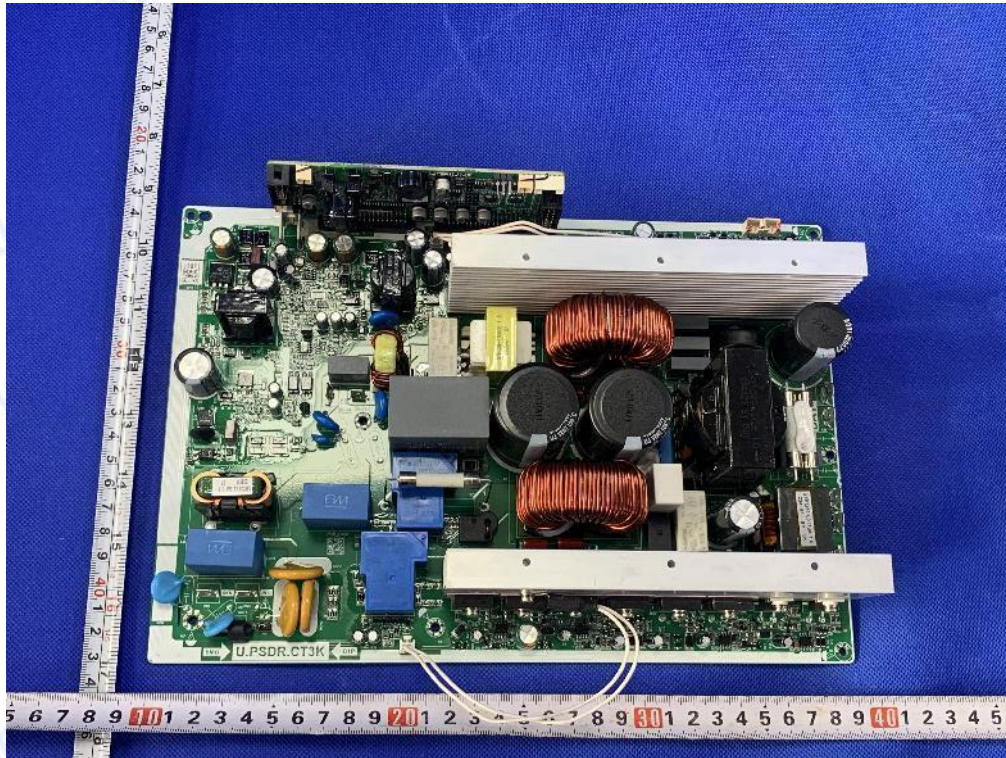
Photo 11: PCB view
